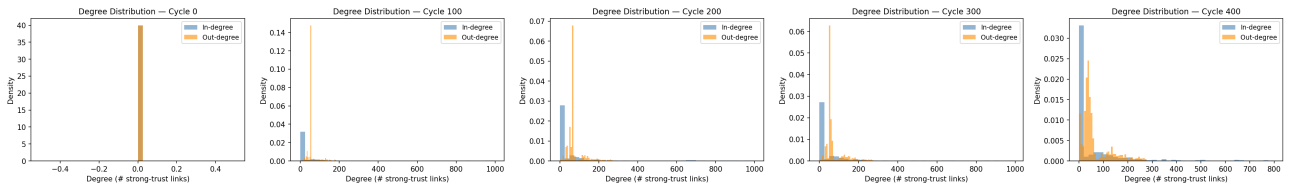
Trust Network Degree Distribution (threshold=0.5)
