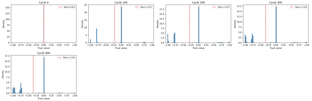
Trust Value Distributions (Faction Polarisation)
