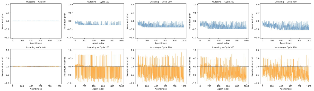
Per-Agent Mean Trust: Outgoing (row) vs Incoming (col)
