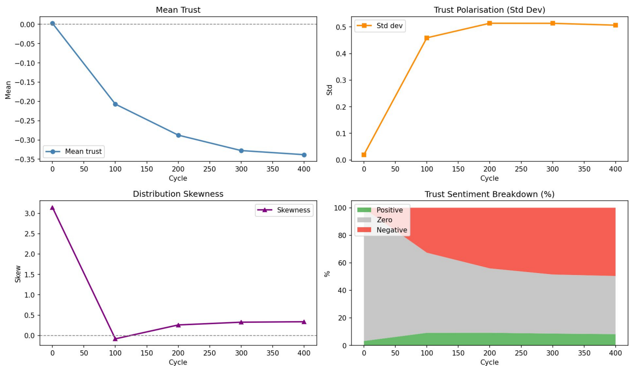
Global Trust Statistics
